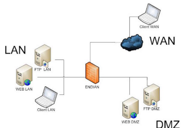
Figura 4 ENDIAN Firewall [5].
